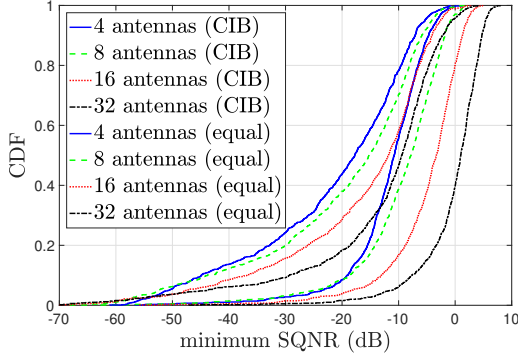
Fig. 3: Empirical CDF of minimum SQNR among 4 users for the proposed CIB and equal combining beamforming vector as the number of transmit antennas is increased. The performance improves as more antennas area added to the BS.
