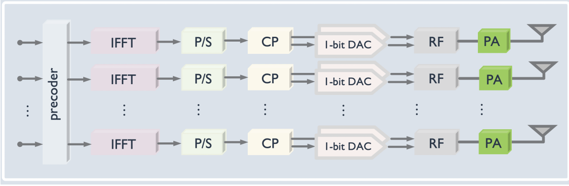
Fig. 1: BS transmitter schematic for multicasting with 1-bit DACs and infinite-resolution ADCs at all active UEs. The BS transmits common data or reference signals to all the active UEs.
